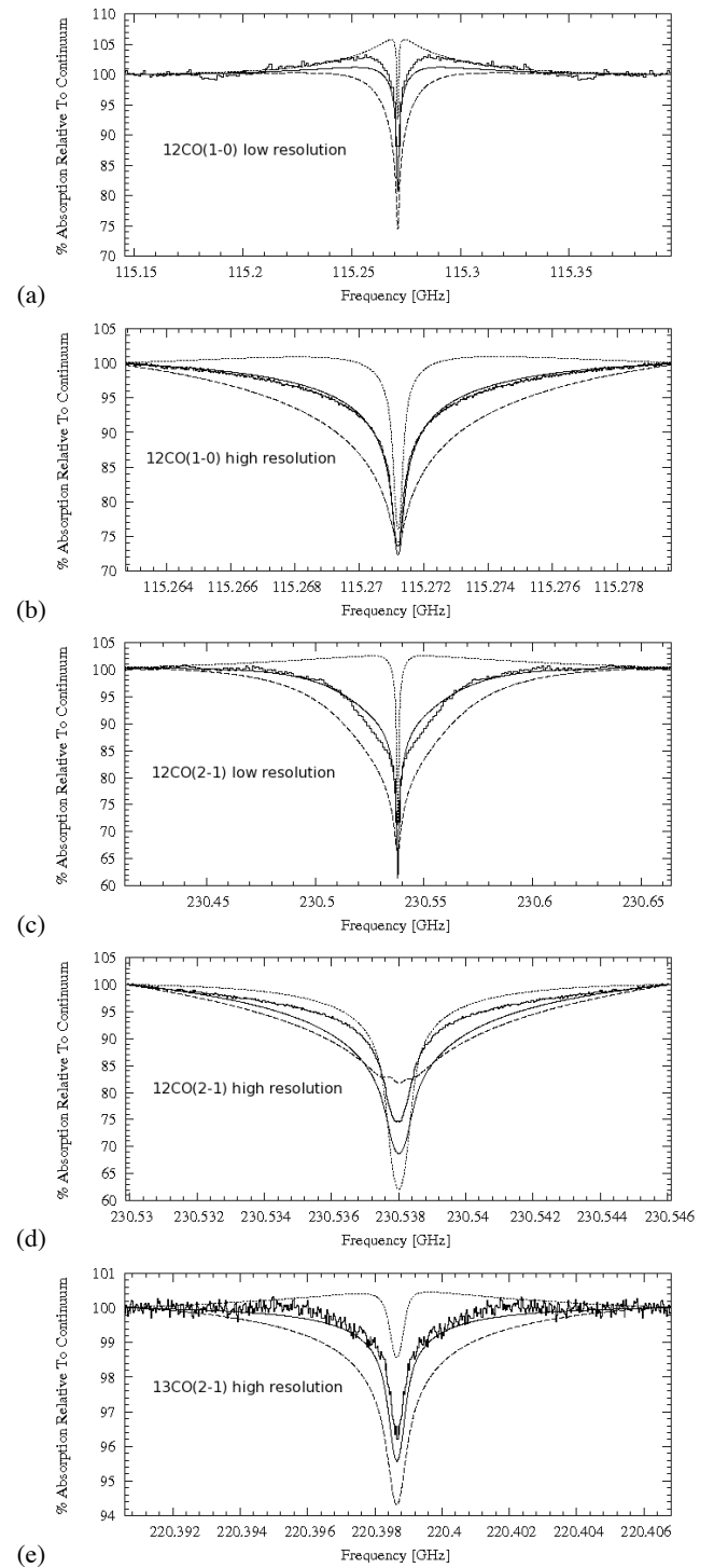
Fig. 7. Same caption as Fig. 6 for 2005.
