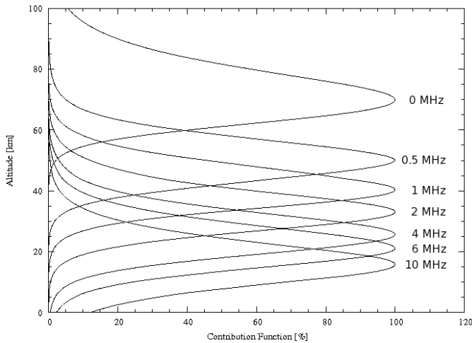
Fig. 3. Contribution functions for the ^{12}CO(2-1) line in 2005. From the highest peak to the lowest one, the frequencies at which the functions are computed are: 0, 0.5, 1, 2, 4, 6 and 10 MHz from the line center. These functions show that it is possible to retrieve the thermal profile between 15 and 70 km from the high resolution ^{12}CO(2-1) line. The ^{12}CO(1-0) line gives similar results. The gap from the surface to 15 km is filled in with the low resolution ^{12}CO(2-1) spectrum because it gives access to the missing part of the spectrum, from 10 MHz from the line center to the continuum.
