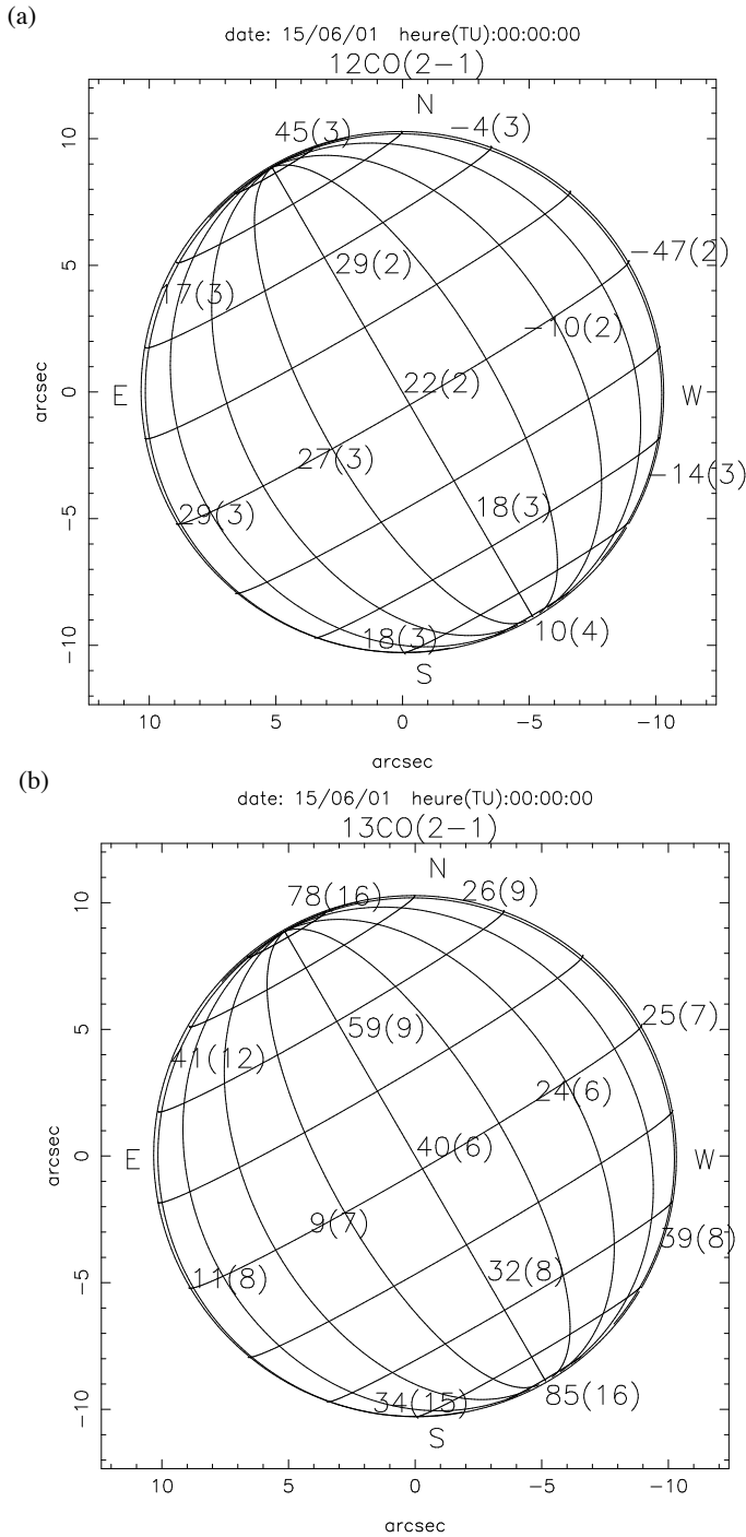
Fig. 16. LOS BI wind velocities [ m.s^{-1} ] for the (a) ^{12}CO(2-1) and (b) ^{13}CO(2-1) observations in 2001. Celestial east/west directions. Parenthese: 1-\sigma fitting uncertainties. Additional uncertainty on each point: 20m.s^{-1} for ^{12}CO(2-1) measurements and 30-40m.s^{-1} for ^{13}CO(2-1) measurements.
