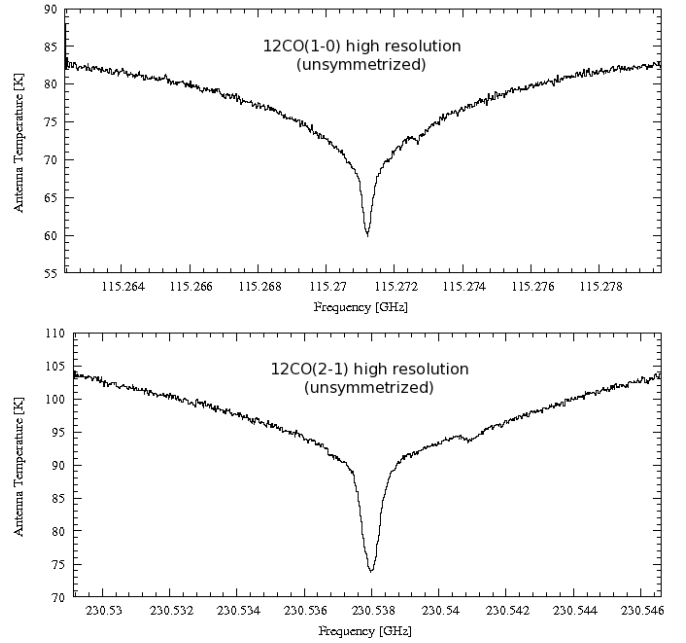
Fig. 2. Antenna temperature spectra of the ^{12}\text{CO}(1-0) and (2-1) lines in 2001 for position 1 with the high spectral resolution mode. The absorption caused by terrestrial mesospheric CO can be seen at 1.5 MHz on the blue wing of the line center of the (1-0) line and 3 MHz on the blue wing of the line center of the (2-1) line.
