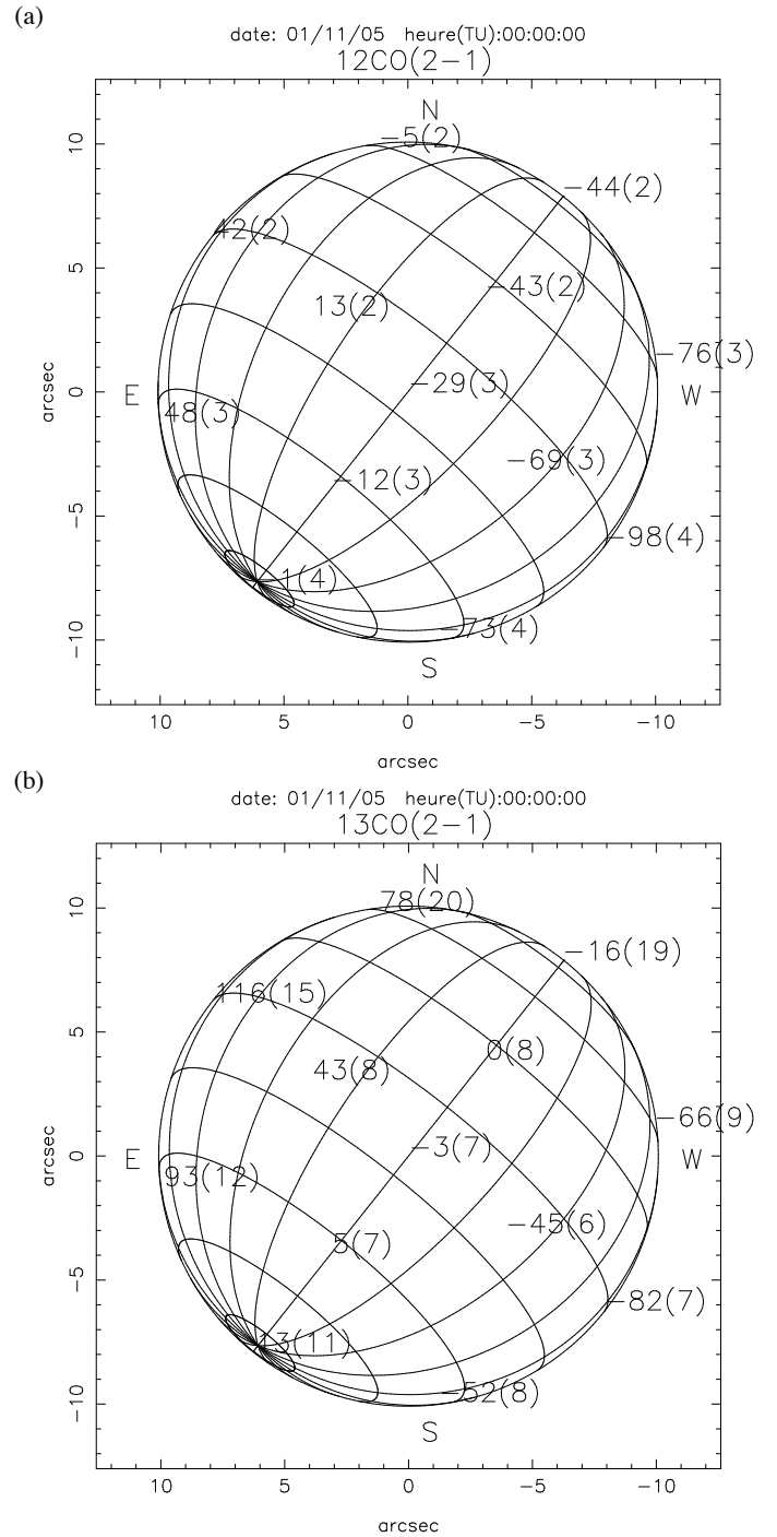
Fig. 17. LOS BI wind velocities [ m.s^{-1} ] for the (a) ^{12}CO(2-1) and (b) ^{13}CO(2-1) observations in 2005. Celestial east/west directions. Parenthese: 1-\sigma fitting uncertainties. Additional uncertainty on each point: 20m.s^{-1} for ^{12}CO(2-1) measurements and 30-40m.s^{-1} for ^{13}CO(2-1) measurements.
