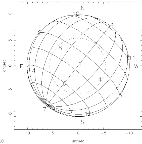
Fig. 1. Geometry of the observations in (a) 2001 and (b) 2005. Positions of observed points are given in Tables 2 and 3. Their position on the disks are only approximative. The field of view (full width at half maximum of the beam) at 230 GHz is plotted in dashed lines for position 1. Celestial east/west directions.
