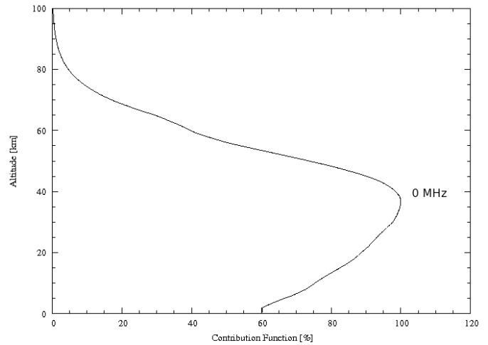
Fig. 4. Contribution function for the central frequency of the ^{13}CO(2-1) line in 2001.
