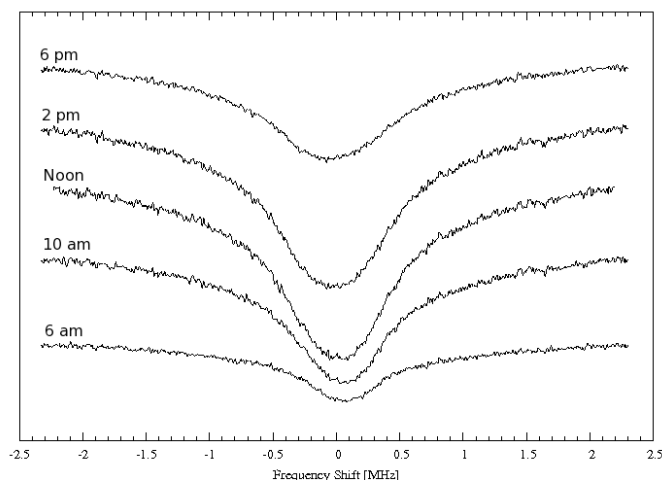
Fig. 15. ^{12}\text{CO}(2-1) line cores in 2005 for five positions on the equator. Positions are: 90W, 30W, Central Meridian (CM), 30E and 90 E and correspond to 6 pm, 2 pm, noon, 10 am and 6 am in local time.
