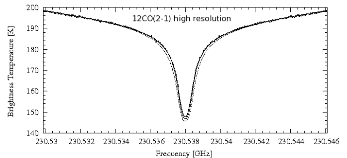
Fig. 5. ^{12}CO(2-1) high resolution line in 2005 fitted with the best fit model (solid line). The dotted model corresponds to an increase of q_{CO} from 8.5 \cdot 10^{-4} to 13.0 \cdot 10^{-4} above 50 km (homopause level).
