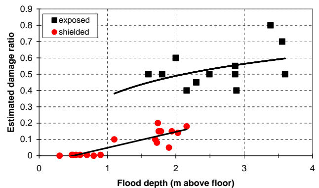
Fig. 16. Damage ratios and fragility curves as a function of inundation depth and exposure for traditional brick buildings with RC columns.
