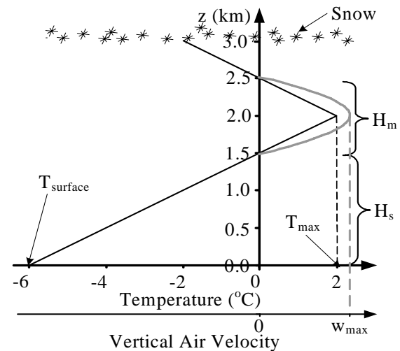
Fig. 3. A schematic diagram of the typical temperature and humidity profile used for this study is shown. H_m is the depth of the melting layer ( T > 0^\circ\text{C} ), H_s is the depth of the subfreezing layer ( T < 0^\circ\text{C} ), T_{\max} and T_{\text{surface}} are the maximum and surface temperatures of the temperature profile. The initial profile of weak ascending air (Eq. 11) from the warm conveyor belt is shown in grey with the maximum vertical air velocity in the middle of the melting layer ( w_{\max} ). Snow is falling at 5 \text{ mm/h} from 3 km above the surface.
