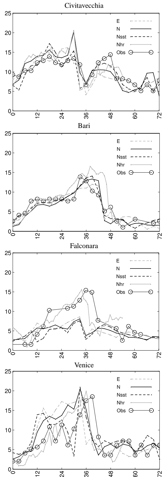
Fig. 13. Time series of surface wind speed. The X-axis shows time, in hours from 3 November 00:00 UTC to 6 November 00:00 UTC. Y-axis shows U_{10} in \text{ms}^{-1} .
