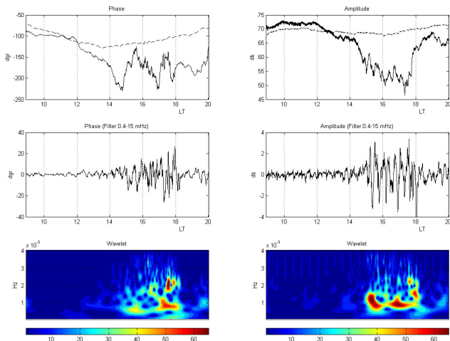
Fig. 3. Phase and amplitude anomalies (top two panels), filtered signals (middle panels) and their wavelets (bottom panels) for 4 November 2004.
