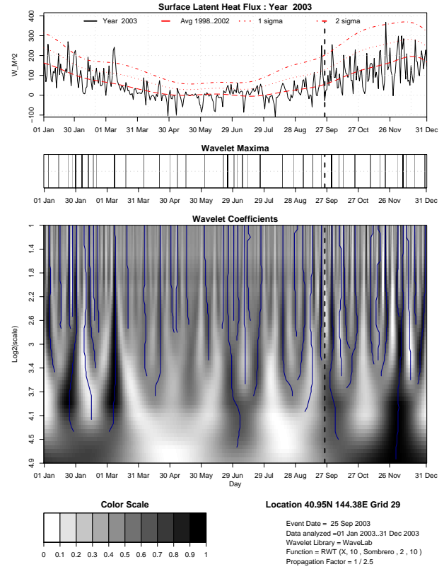
Fig. 2. Wavelet transformation of SLHF data over grid 29 (epicentral region).
