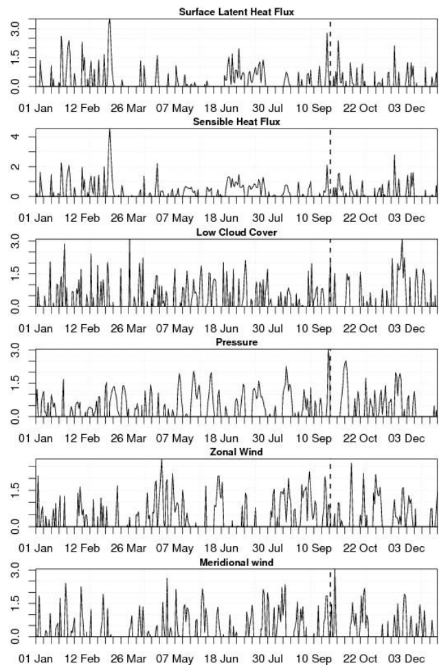
Fig. 5. Various atmospheric and EM anomalies detected prior to the Tokachi earthquake.
