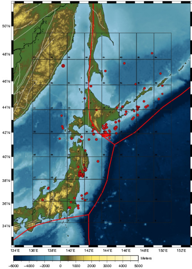
Fig. 1. Map of Japan showing the location of the epicenter (star) of earthquake ( M_w=8.3 ) 25 September 2003. Plate boundaries, faults and their type are also shown. The grids represent the location for which experiments were performed.
