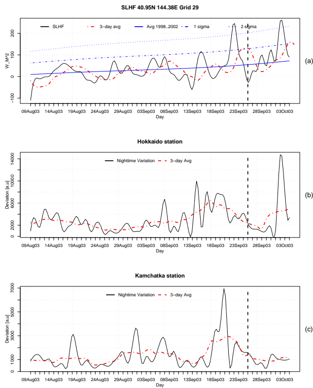
Fig. 4. (a) SLHF (solid line) for the region around 40.95^{\circ} N and 144.38^{\circ} E, its 3-day average (dot full line), the 5-year average (solid trend line) with 1 and 2 sigma. The LF signals observed at Moshiri, Japan ( 44^{\circ} N, 142^{\circ} E) (b) and Petropavlovsk-Kamchatski, Russia ( 53^{\circ} N, 158^{\circ} E) (c), with their respective 3-day average for August to October 2003.
