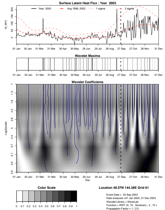
Fig. 3. Wavelet transformation of SLHF data over grid 61 (Kamchatka station).
