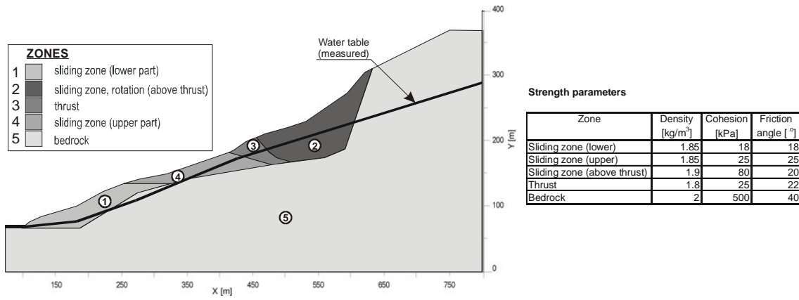
Fig. 4. Division of the slope into geotechnical zones.
