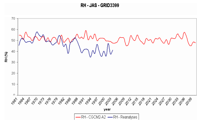
Fig. 8. Summer values of Relative humidity.
