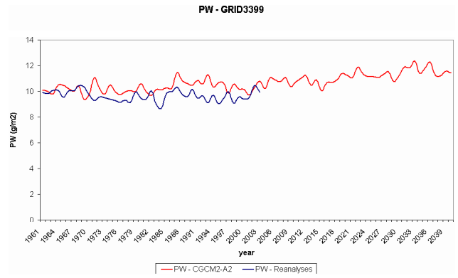
Fig. 4. Annual values of Precipitable Water.
