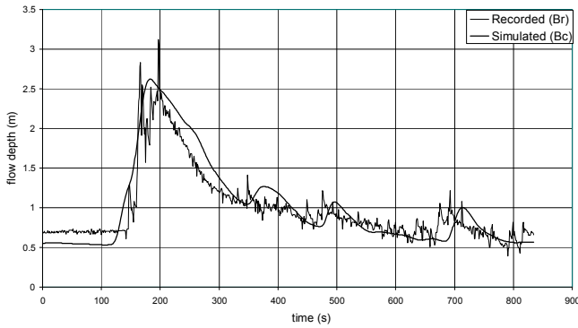
Fig. 3. Comparison between recorded flow depth in the second gauge station and simulated one.
