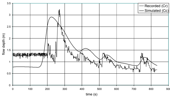
Fig. 4. Comparison between recorded flow depth in the third gauge station and simulated one.
