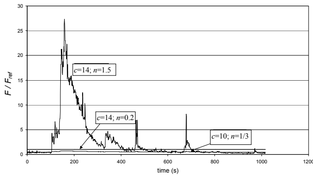
Fig. 6. Impact forces. F_{ref} is the component of the impact force when c and n are the same as those used in the simulation.
