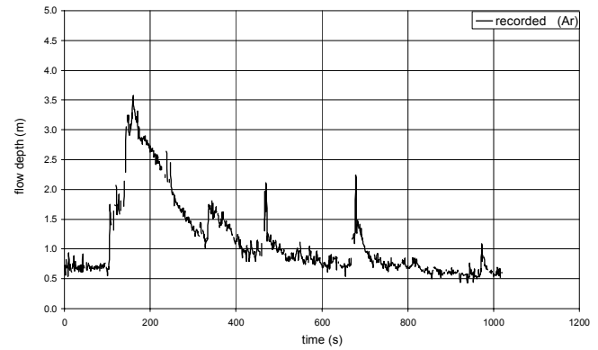
Fig. 2. Recorded flow depth at the upstream gauging station.
