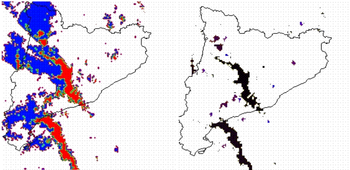
Fig. 3. Example of application of the 2-D algorithm. (a) Convective system, in which red areas are “convective” rainfall regions, while blue means “stratiform” rainfall; (b) convective precipitation areas have been isolated. The example corresponds to the 10 June 2000 event (00:00 UTC).
