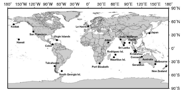
Fig. 2. The locations of the 1883 Krakatau tsunami recording.
