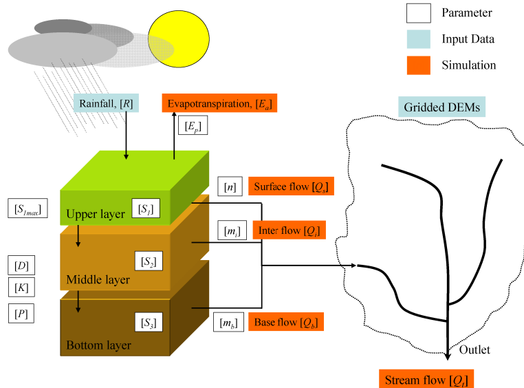
Fig. 2. Schematic diagram of the 3-layer TOPMODEL.
