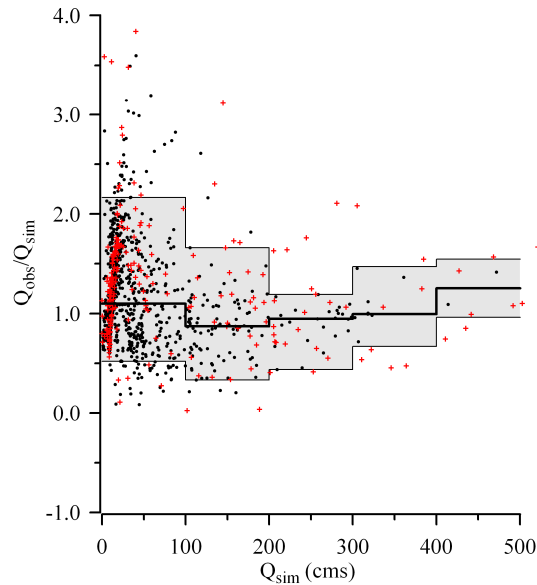
Fig. 6. the scatter plots of the Q_{\text{obs}}/Q_{\text{sim}} against Q_{\text{sim}} . The black circle and red cross markers represent the calibration and validation events. The black lines and the gray zones are the median and 90% confidence interval derived from all calibration events.
