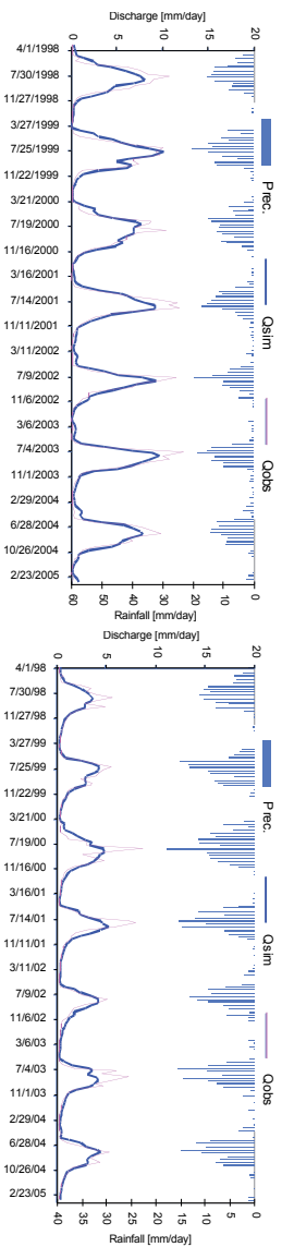
Fig. 3. Simulated and observed stream flow hydrographs for the 15-days time step models (CR III).
