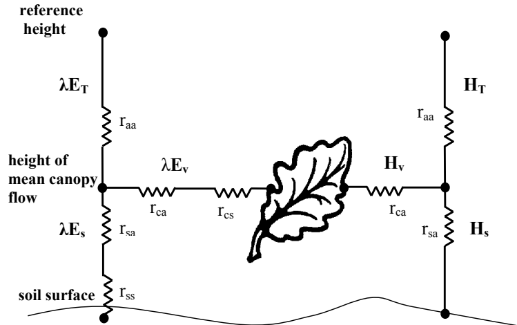
Fig. 6. Schematic of the Shuttleworth-Wallace (1985) two-component canopy model.
