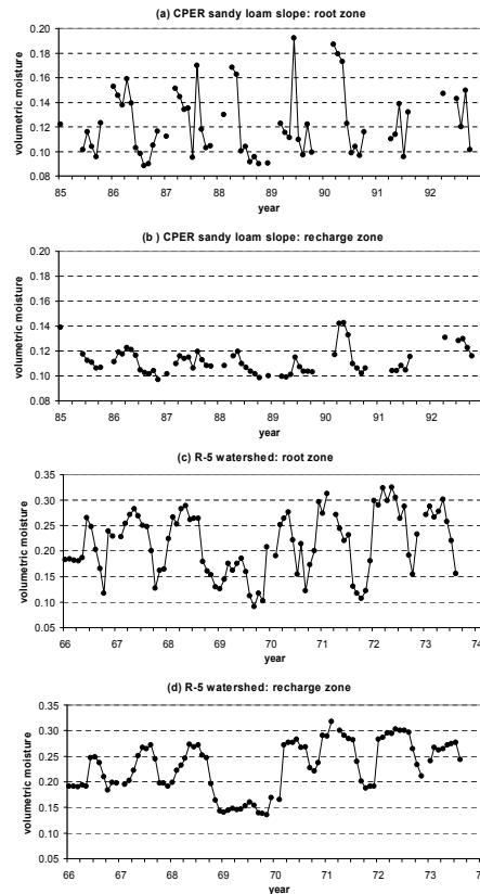
Fig. 7. Monthly averages of observed volumetric soil moisture at the two grassland sites: (a) root zone at the CPER (measurements made at depths of 30 and 45 cm), (b) recharge zone at the CPER (measurements made at depths of 60, 75 and 90 cm), (c) root zone at the R-5 watershed (measurements made at depths of 15, 30, 45 and 60 cm), and (d) recharge zone at the R-5 watershed (measurements made at depths of 75, 90, 105 and 120 cm).
