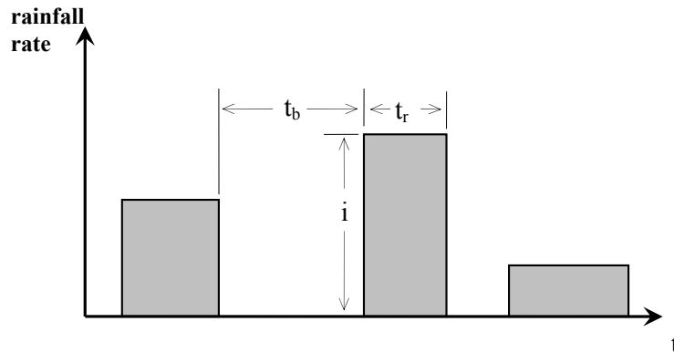
Fig. 1. The rectangular pulse model of precipitation.
