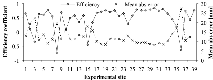
Fig. 5. Efficiency coefficients and values of mean absolute error between measured and modelled snow water equivalent in 39 measurement sites.
