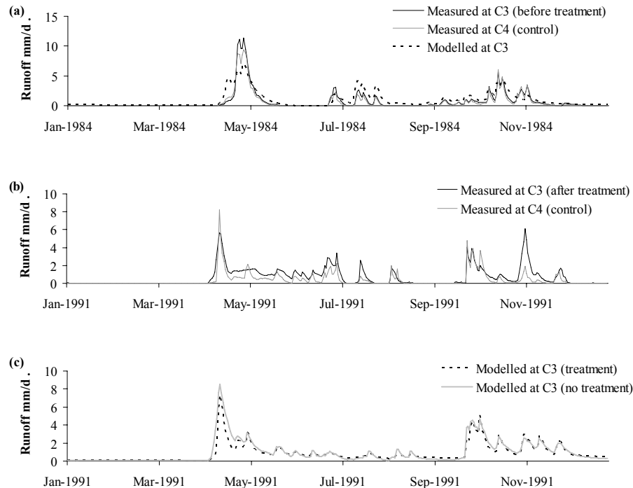
Fig. 11. Measured runoff from catchments C3 and C4, and modelled runoff from catchment C3 in 1984 (a) , measured runoff from catchments C3 and C4 in 1991 (b) , and modelled runoff from catchment C3 with and without ditch cleaning (c) . Ditch cleaning was conducted in 1989.
