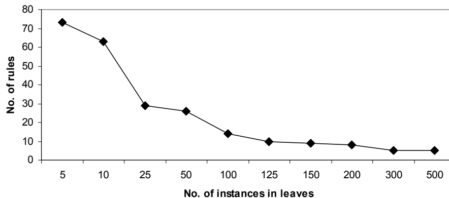
Fig. 3. Size of the generated regression trees.
