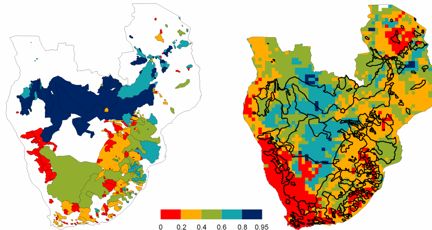
Fig. 11. Baseflow indices at discharge observation stations in Southern Africa, mapped onto the pertaining basins (Bullock et al., 1997, their Fig. 4.35) (left); groundwater recharge as a fraction of total runoff from land as computed with WGHM, with polygon outlines of Bullock et al. (1997) for easier comparison (right). Please note that the polygon outlines are not basin boundaries but boundaries of polygon with the same color in the figure on the left.
