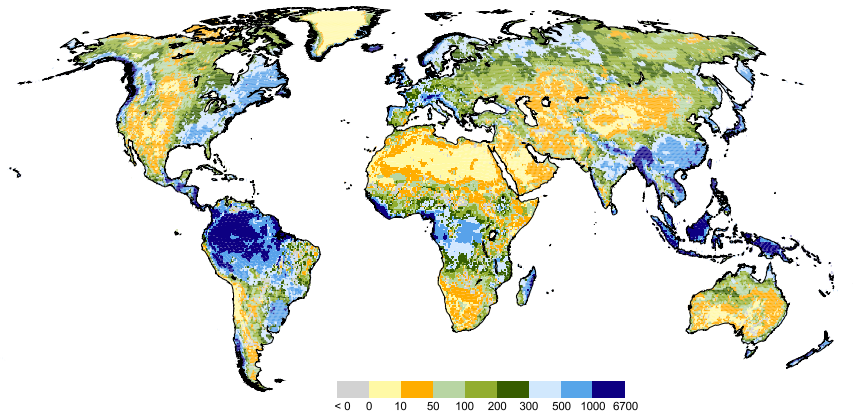
Fig. 7. Long-term average total runoff from land and open water fraction of cell, in mm/yr, for the time period 1961–1990, as computed by WGHM (ensemble mean using GPCC/CRU precipitation).
