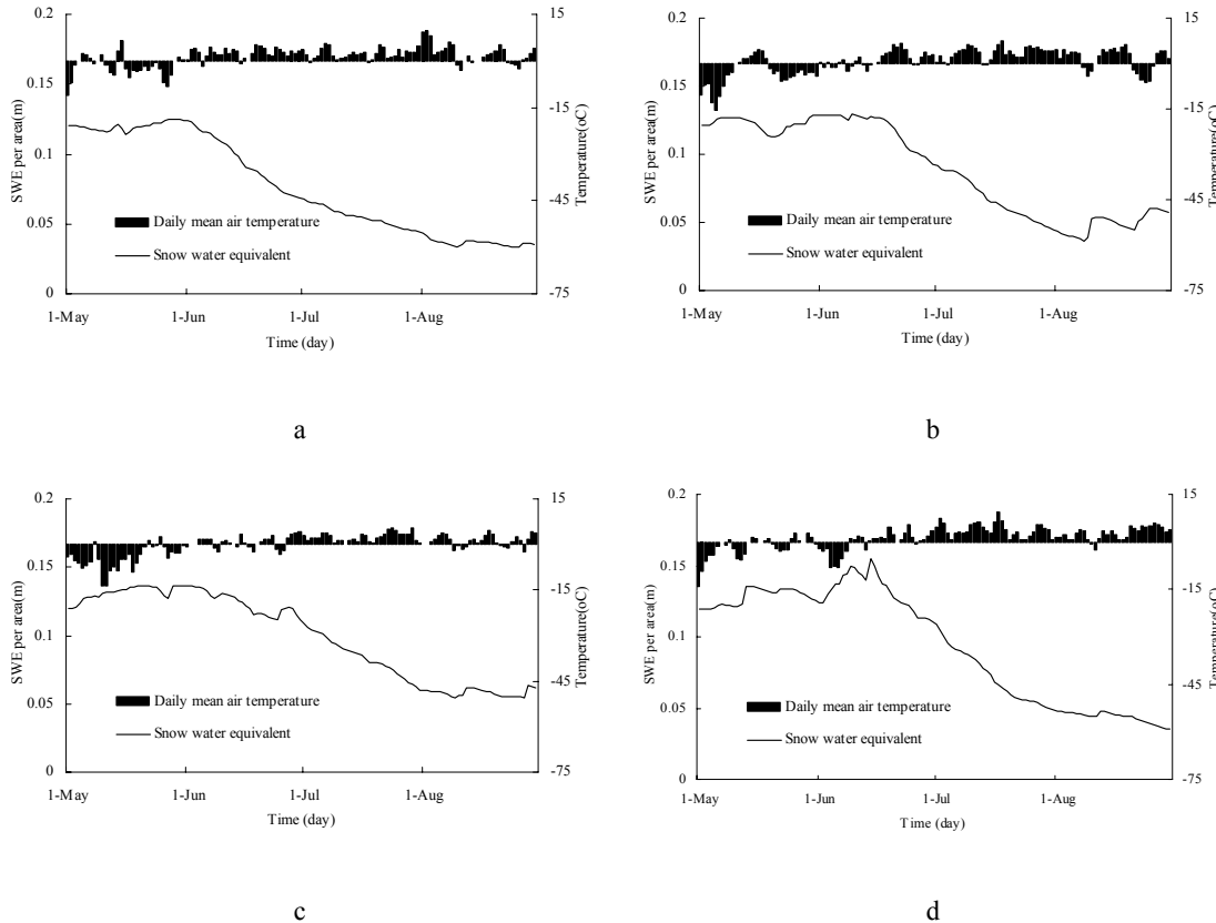
Fig. 12. Model calibration results (4) (a), (b), (c), and (d) are daily SWE depletion/accumulation curve with daily mean air temperature for 1990, 1991, 1993, and 1994.
