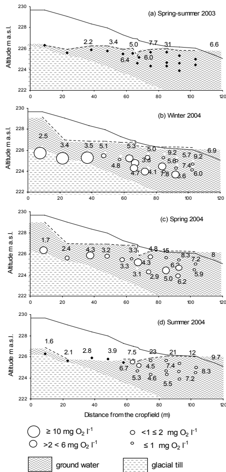
Fig. 11. Mean DOC concentrations ( \text{mg l}^{-1} ) along the studied transect and dissolved oxygen ranges during: (a) March–August 2003, (b) December–March 2004, (c) April–May 2004 and (d) June–July 2004.
