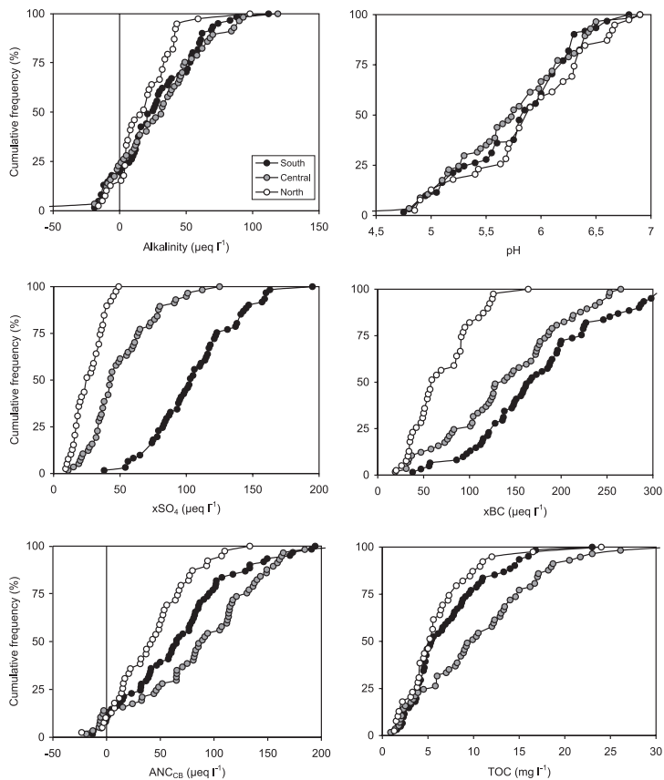
Fig. 2. Cumulative frequency distributions (%) for Gran alkalinity, pH, \text{xSO}_4 , \text{xBC} , \text{ANC}_{\text{CB}} and TOC of lakes in south ( \bullet ), central ( \circ ) and north ( \circ ) Finland. The value for a lake is the median in 1990–2003.
