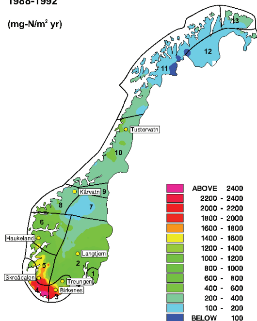
Fig. 1. Total deposition of nitrogen (oxidized + reduced) 1988–1992 (maximum total Nr deposition in the monitoring period) and 1997–2001 (minimum total Nr deposition in the monitoring period) in mainland Norway. The unit is mg N/m 2 year. From Hole and Tørseth (2002). Precipitation zones from Hanssen-Bauer (2005) are also indicated.
