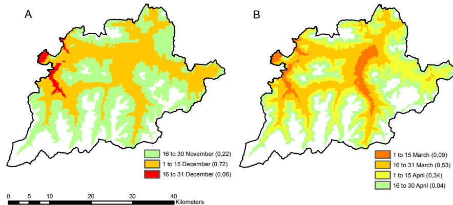
Fig. 6. Weighted optimal start of the winter season ( A ) and weighted optimal end of the winter season ( B ) for the water logistic system of the study area Kitzbueheler region, as the result of equation (3). The weighted values (between brackets) are relative to the number 1.
