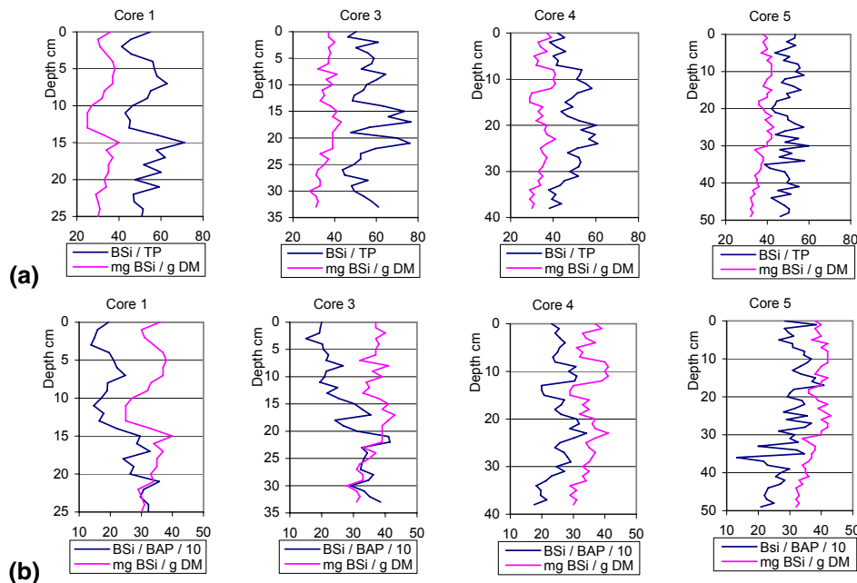
Fig. 4. (a) BSi and the ratio BSi/TP and (b) BSi and the ratio BSi/BAP vs. depth in the cores 1, 3, 4 and 5. A peak in the ratios BSi TP -1 and in BSi BAP -1 and a peak in BSi at the same level may indicate epilimnic Si depletion. If the following BSi decrease depends on Si deficit, the P content is not the limiting factor for diatom production and other vegetation may take advantage of the nutritious water. The decrease between 14 and 10 cm in core 1 represents the years of construction 1951–1953 with a very high sediment accumulation rate and does not show the epilimnic nutrient conditions. The graphs start about 1850.
