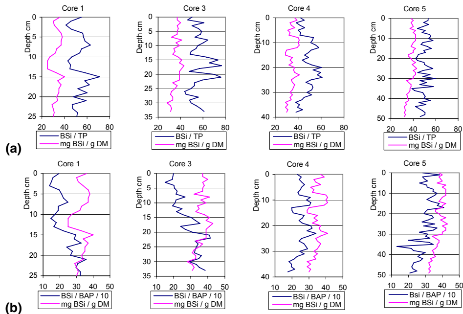
Fig. 4. (a) BSi and the ratio \text{BSi}/\text{TP} and (b) BSi and the ratio \text{BSi}/\text{BAP} vs. depth in the cores 1, 3, 4 and 5. A peak in the ratios \text{BSi}/\text{TP}^{-1} and in \text{BSi}/\text{BAP}^{-1} and a peak in BSi at the same level may indicate epilimnic Si depletion. If the following BSi decrease depends on Si deficit, the P content is not the limiting factor for diatom production and other vegetation may take advantage of the nutritious water. The decrease between 14 and 10 cm in core 1 represents the years of construction 1951–1953 with a very high sediment accumulation rate and does not show the epilimnic nutrient conditions. The graphs start about 1850.
