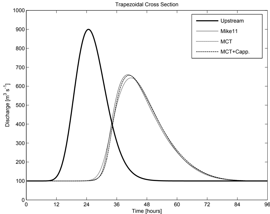
Fig. 12. Comparison, for the trapezoidal cross section, of the MIKE11 resulting discharges (thin solid line) with the ones obtained using the new MCT scheme (dotted line) and the new scheme with the Cappalaere (1997) correction (dashed line). The upstream inflow wave is shown as a thick solid line.
