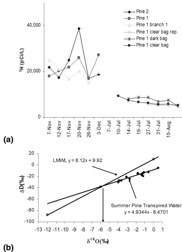
Fig. 2. (a) Summer and winter Tritium concentrations in transpired waters collected from pine trees growing approximately 300 m south of the National Tritium Labeling Facility at Berkeley, California. (b) Stable isotope ratios in pine transpired water samples collected during 7 July to 15 August 1995.
