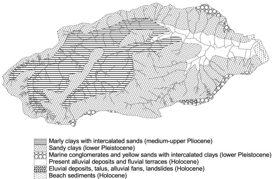
Fig. 2. Geo-lithological scheme.
