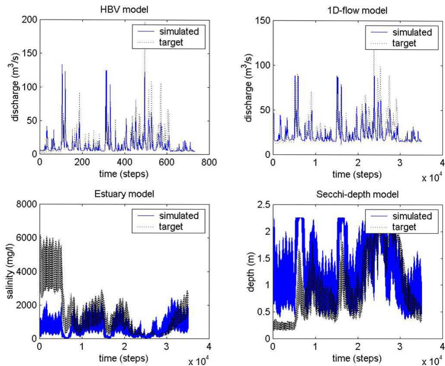
Fig. 7. Results connected models.
