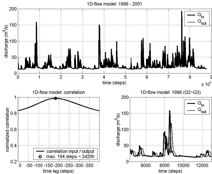
Fig. 2. 1-D-flow model.
