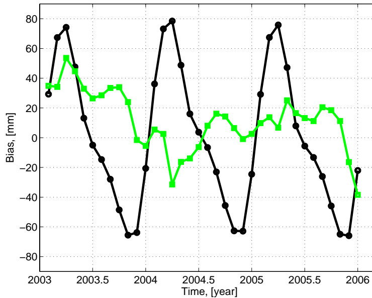
Fig. 9. Time series of bias computed on the basis of the CPC-LDAS (black circles) and the differences between the bias from CPC-LDAS and LEW (green squares) for the upper Zambezi target area.
