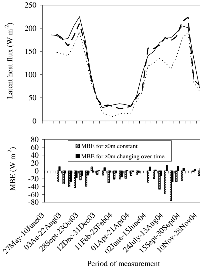
Fig. 10. Comparison between the performance of the standard (dashed line) and the improved NOAH LSM (bold dashed line). The solid line corresponds to the observed latent heat flux.
