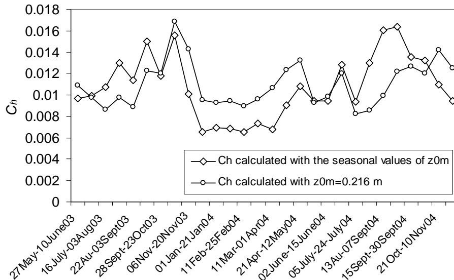
Fig. 7. Comparison between the surface exchange coefficients for heat calculated with the seasonal values of z_{0m} and with a fixed value of 0.216 m.
