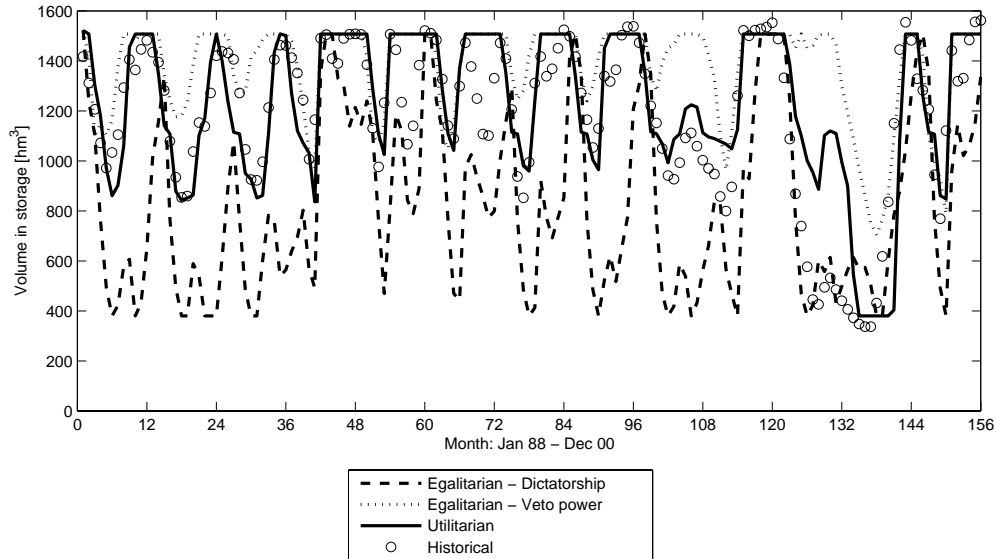
Fig. 2. Simulated storage levels for different group-decision making approaches.
