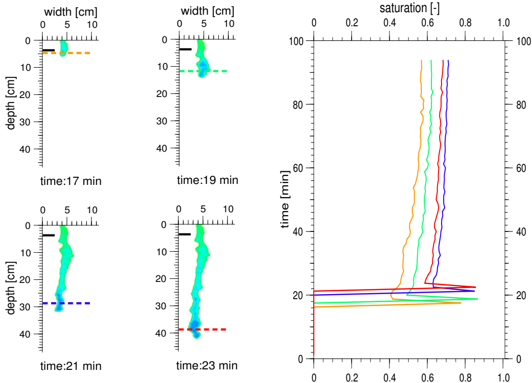
Fig. 9. The temporal dynamics of water saturation inside the finger core during the passage of a finger at different depths. Note the minimum of water saturation behind the tip and the slow increase of water saturation until a quasi-stable state is reached.
