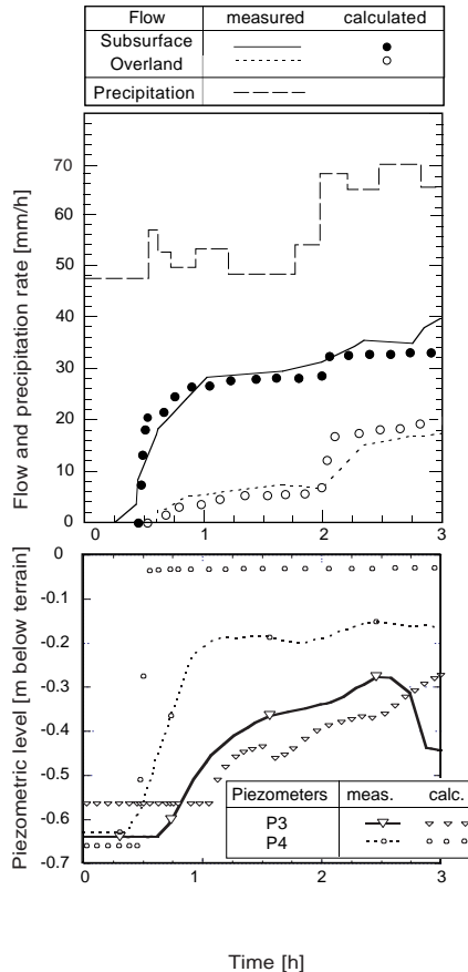
Fig. 3. Measured flows and examples of the piezometer and tensiometer measurements of the third experiment at Willerzell Hang (site 18). Subsurface flow started before overland flow and was more intense than overland flow. The corresponding results of the calculations with the numerical QSOIL model are also shown (dots).
