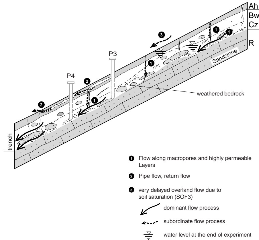
Fig. 4. Hillslope profile of Willerzell Hang, showing the identified flow processes.
