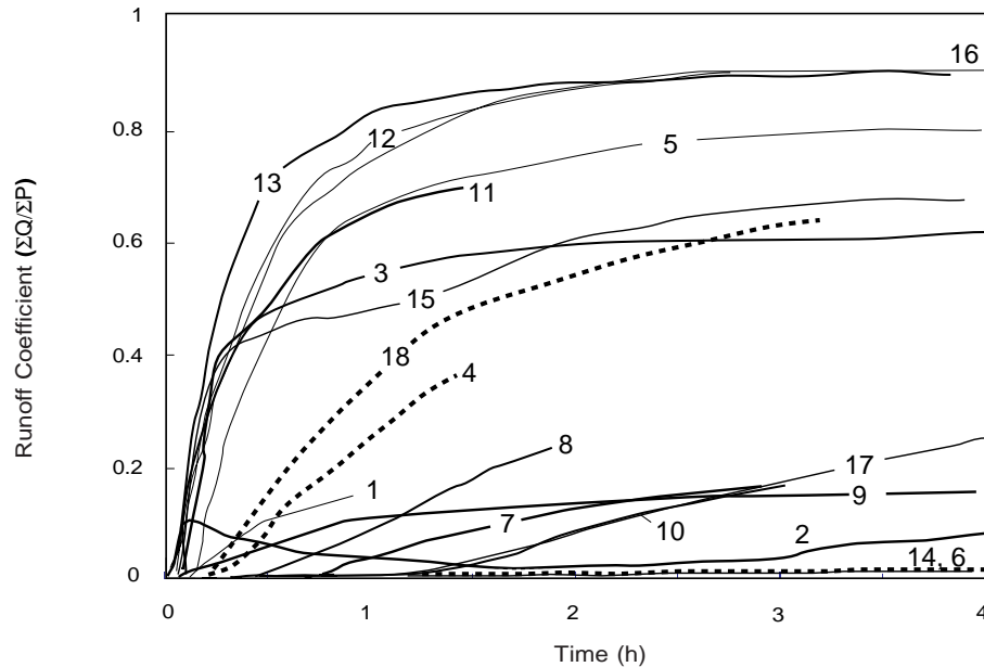
Fig. 6. The volumetric runoff coefficients (cumulated runoff divided by cumulated precipitation) observed at the 18 sites when sprinkling of 50 to 100 mm/h on the initially dry soils was applied. Solid lines indicate the dominance of overland flow processes, dashed lines subsurface flow dominance. The numbers refer to the site numbers as listed in Table 1.
