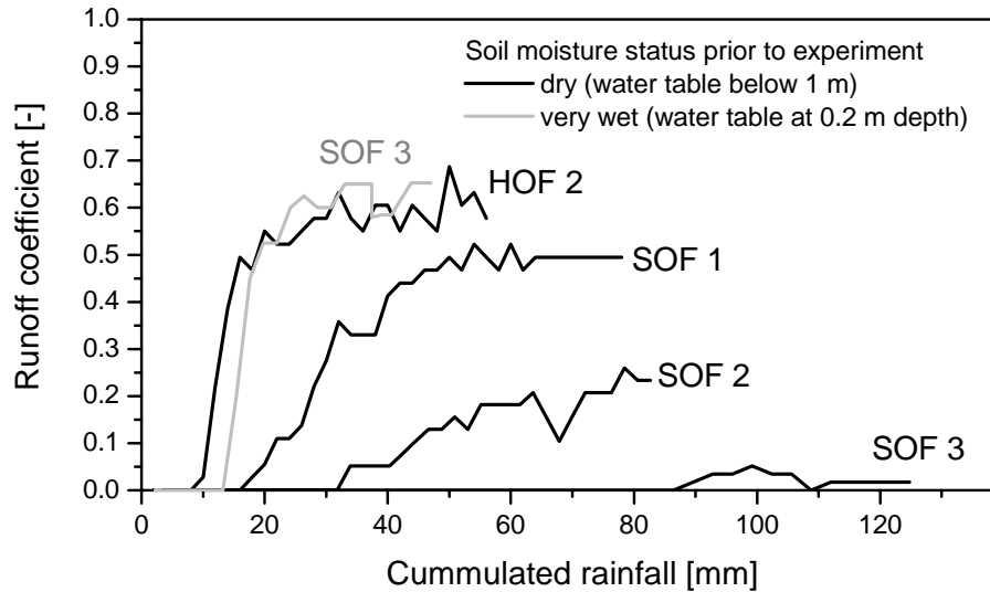
Fig. 4. Runoff coefficients observed during sprinkling experiments over 1 m 2 with an intensity of 60 mm/h on agricultural fields (HOF 2) and grassland (SOF 1 to 3).
