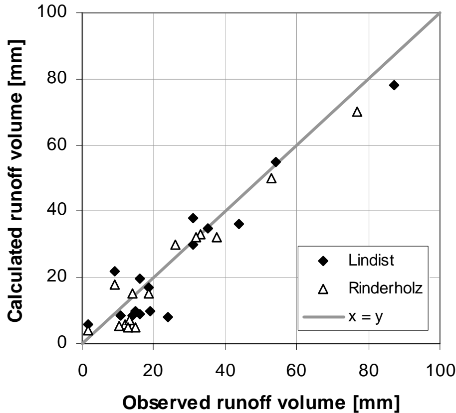
Fig. 11. Observed and calculated runoff volumes for all flood events between summer 2001 and fall 2003 with a specific peak discharge larger than 0.2 \text{ m}^3 \cdot \text{s}^{-1} \cdot \text{km}^{-2} in Lindist and Rinderholz.
