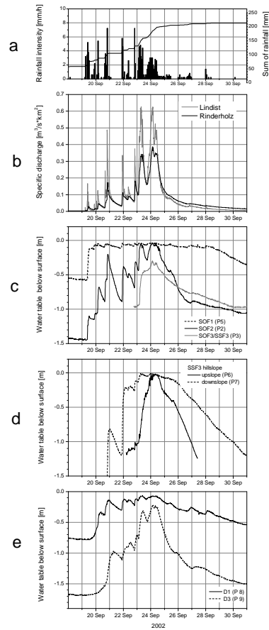
Fig. 3. Rainfall (a), catchment runoff (b) and soil-water levels measured in different process areas (c)–(e) in the Lindist and Rinderholz sub-catchments during the September 2002 flood event.
