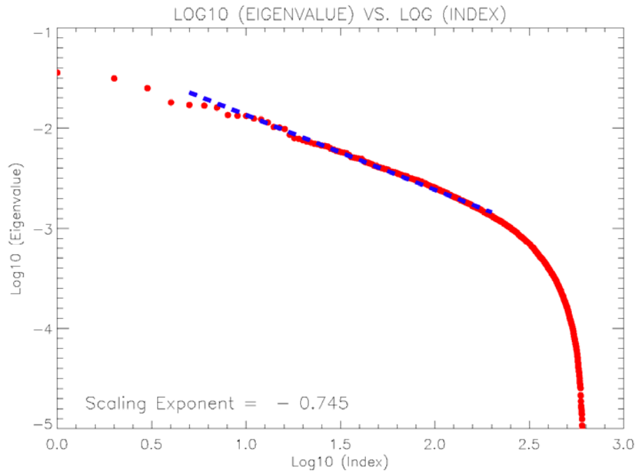
Fig. 4. Plot of the eigenvalue spectrum p_n on a log-log plot. \text{Log}_{10}p_n is plotted as a function of \text{Log}_{10}n , where n is the index number of the eigenvector ( n=1 has the largest value of p_n , and the rest are ordered by descending values of p_n ).
