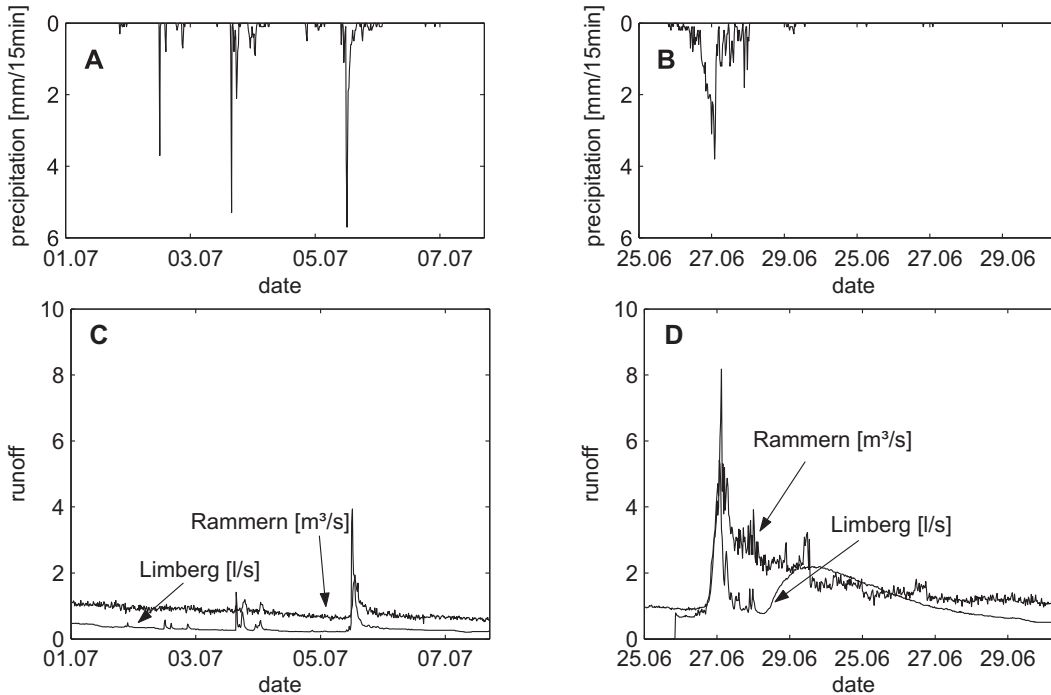
Fig. 2. Typical hydrographs of the micro-scale catchment at stream gauge Limberg and meso-scale catchment at stream gauge Rammern: direct and synchronic runoff peaks (C) during short and intensive rainstorms (A), and bimodal runoff events (D) during and after moderate and much longer rainfall events (B) (Kirnbauer et al., 2001, modified).
