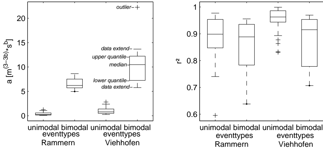
Fig. 11. Boxplots of coefficient a (left) calculated with the nonlinear model with goodness of curve fit r^2 (right) for the two event types at the small-catchment scale (gauge Rammern) and at the meso-scale (gauge Viehhofen).
