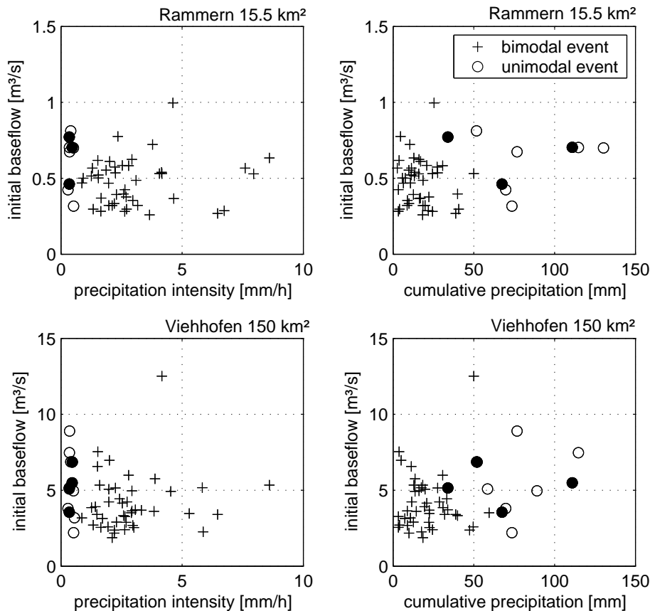
Fig. 12. Initial base flow versus cumulative precipitation, and initial baseflow versus precipitation intensity, for gauge Rammern and Viehhofen (filled circles indicate bimodal events with underpredicted precipitation due to errors in time series).
