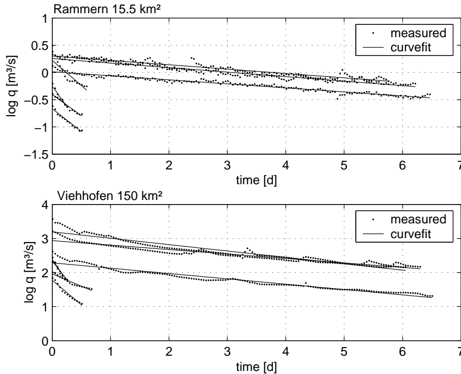
Fig. 8. Recession curves for the rainfall runoff events measured 1997 (every fourth measured point is plotted) for Rammern and Viehhofen: linear model.
