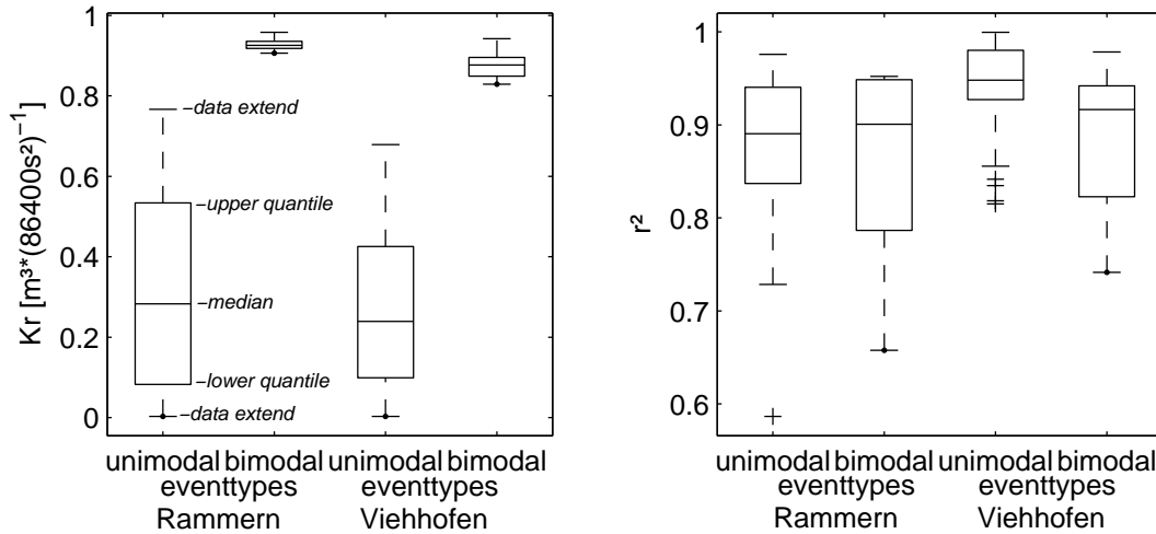
Fig. 10. Box plots of recession coefficients K_r (left) with goodness of curve fit r^2 (right) for the unimodal and bimodal event types at the small-catchment scale (gauge Rammern) and at the meso-scale (gauge Viehhofen).
