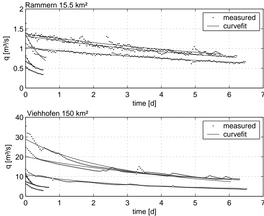
Fig. 9. Recession curves for the rainfall runoff evens measured 1997 (every fourth measured point is plotted) for Rammern and Viehhofen: nonlinear model.
