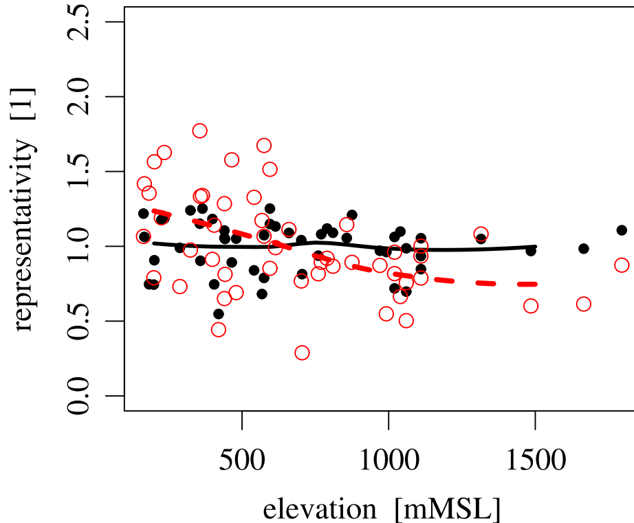
Fig. 5. Relative representiveness in geographical (black bullets) and \gamma -statistical (red circles) distance of the observing stations of set 50. The solid black and dashed red lines are local polynomial regression fits to the bullets and circles, respectively.
