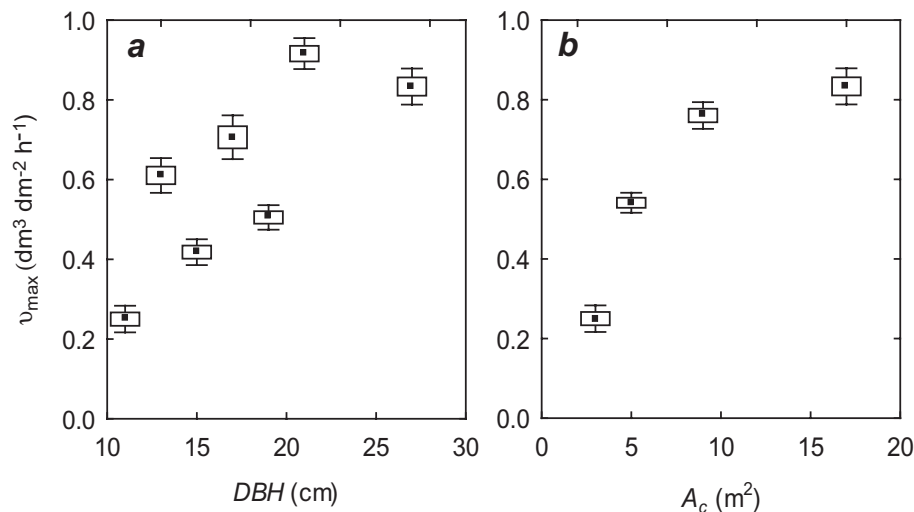
Fig. 1. Relationship between maximum sap velocity ( v_{max} ) and (a) DBH and (b) crown projected area ( A_c ) for P. sylvestris . Individual trees are grouped in integer categories of the independent variable. Points are means, boxes are standard errors and whiskers are 95% confidence intervals.
