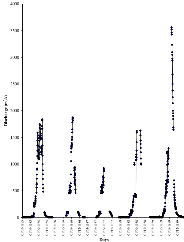
Fig. 2. Daily Hydrograph at Sabari on the Oti River (1985–1989). Typical pattern of Gaps considered in the Spatio-temporal Modelling.
