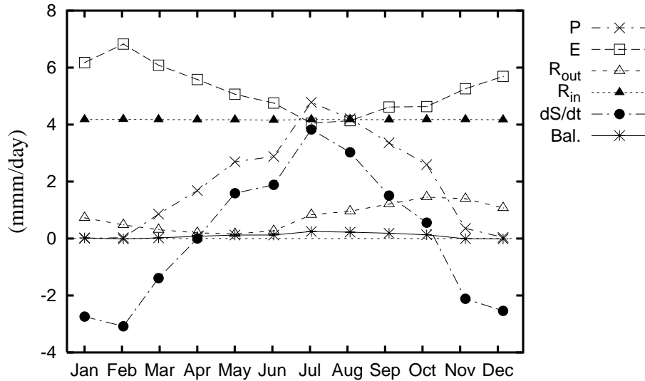
Fig. 10. Hydrological balance over the Sudd wetland in mm/day computed with the calibrated RACMO model (mean annual cycle 1995 to 2000).
