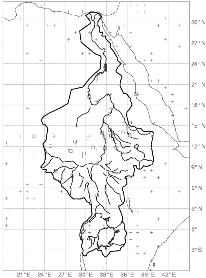
Fig. 5. Location of the precipitation stations (+GPPC, □ Sudan gauging stations).
