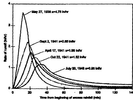
Hydrographs for 22 acre Catchment
