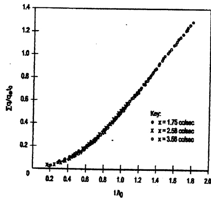
Fig. 5. Laboratory study of overland flow.
