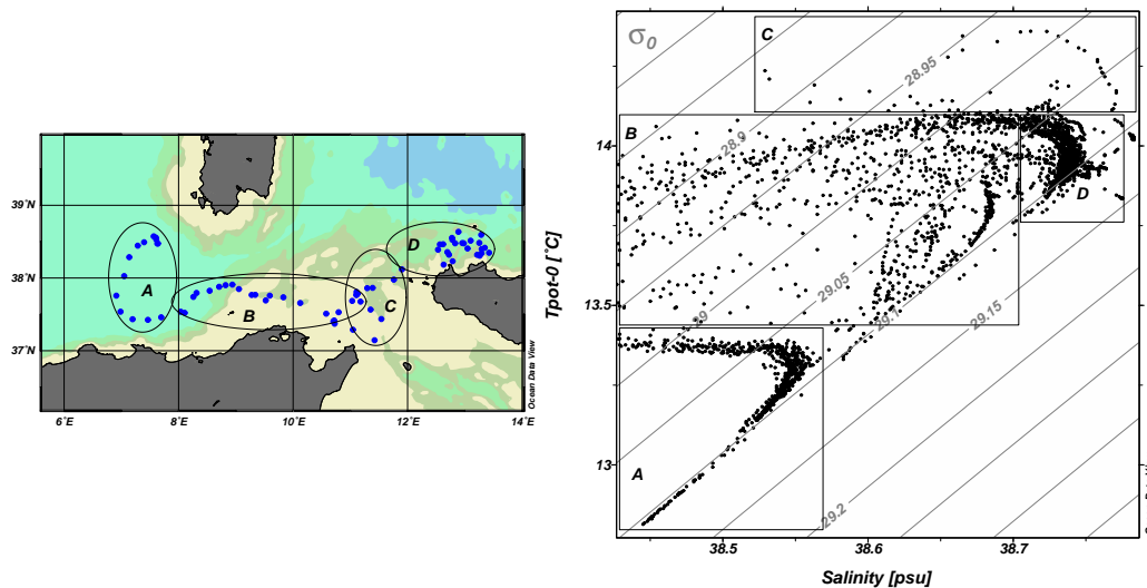
Fig. 3. Float PROVOR 6900294 trajectory and \theta, S curve.
