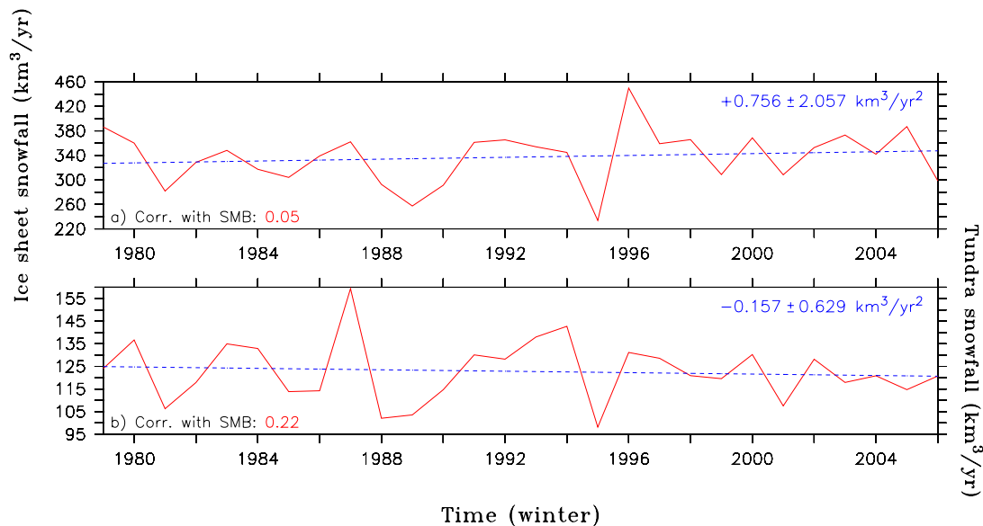
Fig. 11. Time series of the winter (from 1 October YEAR-1 to 30 April YEAR) snowfall before the considered year (in km 3 yr -1 ) over (a) the ice sheet and (b) the tundra. The correlation with the SMB (Fig. 4) is indicated.
