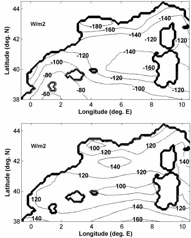
Fig. 2. Spatial distribution of Net Heat Flux from ECMWF 1979–1993 reanalysis data: February (upper panel) and August (lower panel). Units are \text{W/m}^2 .
