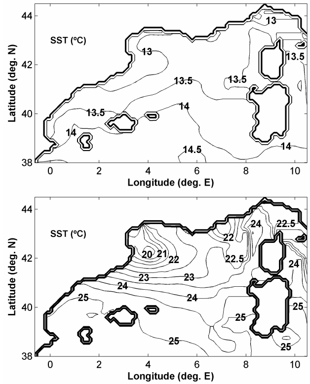
Fig. 5. Sea Surface Temperature (SST) from MED6 monthly climatology: February (upper panel) and August (lower panel). The contour interval is 0.5°C.
