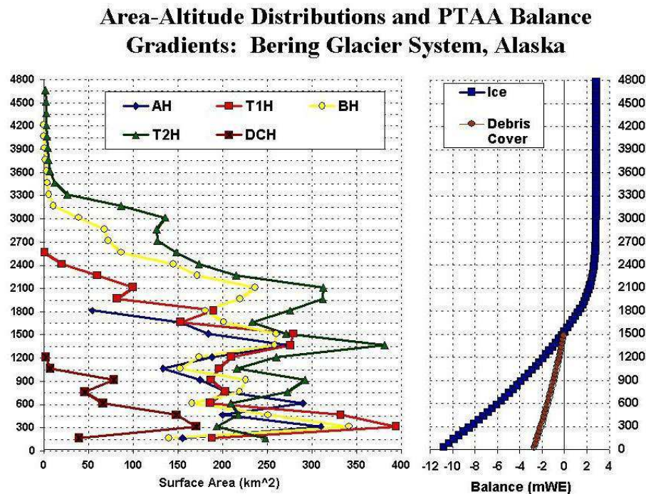
Fig. 8. Area-altitude distributions of four Bering Glacier System outlines and the PTAA mass balance gradients. The graph on the left shows Bering Glacier System surface area within 150 m elevation bands for each of the four outlines and debris cover. The graph on the right is the average (1950–2004) PTAA modeled mass balance gradient.
