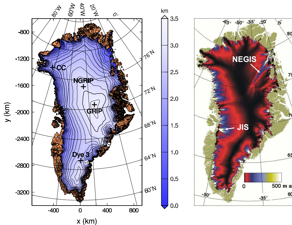
Fig. 1. Present-day Greenland ice sheet. Left panel: Observed surface topography (data by Bamber et al., 2001). Labels in km a.s.l., contour spacing 200 m. “Icy” hues indicate glaciated land, whereas brown areas are ice-free. Right panel: Balance velocities (plot by Bamber et al., 2001). The north-east Greenland ice stream (NEGIS) and the Jakobshavn ice stream (JIS) are clearly visible.
