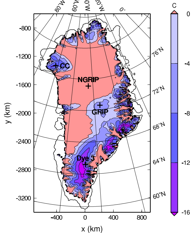
Fig. 10. Best-agreement simulation (run #3): Present-day basal temperature (relative to the pressure melting point). Red areas are at the pressure melting point.
