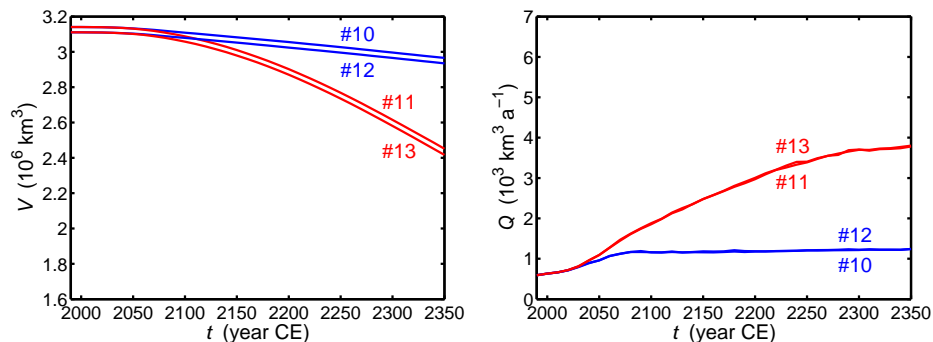
Fig. 12. Simulated evolution of the ice volume V and the freshwater discharge Q for the global warming runs #10 (no NEGIS, WRE450), #11 (no NEGIS, WRE1000), #12 (NEGIS/ m=3 , WRE450) and #13 (NEGIS/ m=3 , WRE1000). Note that blue and red curves correspond to the WRE450 and WRE1000 scenarios, respectively.
