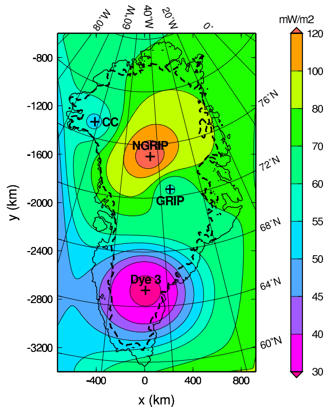
Fig. 3. Distribution of the geothermal heat flux based on Pollack et al. (1993) and the values of Eq. (1) for the ice-core sites GRIP, NGRIP, Camp Century and Dye 3. The heavy dashed line indicates the present-day ice margin.
