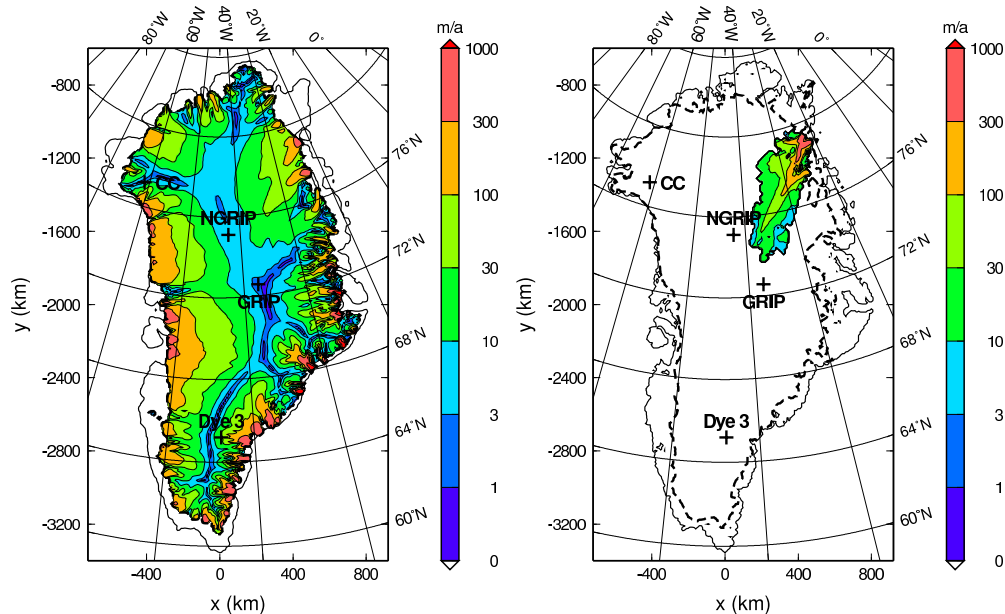
Fig. 9. Simulated (left panel; best-agreement run #3) vs. observed (right panel; Joughin et al., 2001 ; NEGIS area only) present-day surface velocities.
