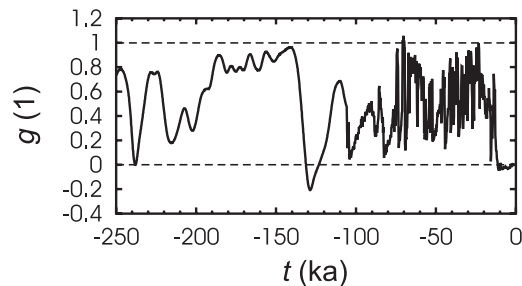
Fig. 2. Glacial index g , based on surface-temperature histories from the Greenlandic GRIP \delta^{18}\text{O} record from today back until 105 ka ago, and from the Antarctic Vostok \delta\text{D} record prior to 105 ka ago.
