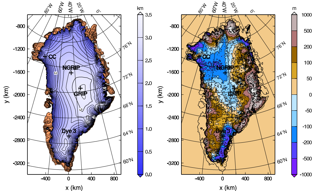
Fig. 4. Reference simulation (run #1): Present-day surface topography (left panel; contour spacing 200 m, labels in km a.s.l.), and difference between simulated and observed present-day ice thickness (right panel). The heavy dashed lines indicate the simulated (left panel) and observed (right panel) ice margins.
