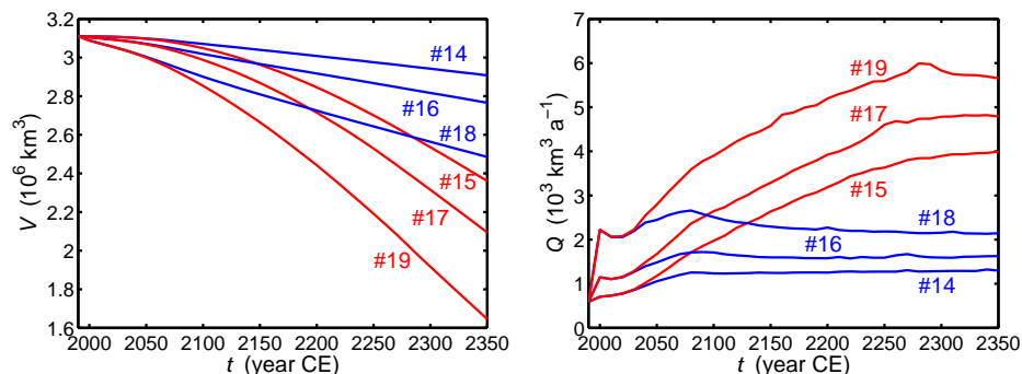
Fig. 13. Simulated evolution of the ice volume V and the freshwater discharge Q for the global warming runs #14 (NEGIS/ m=3 , WRE450, \gamma=0.1 \text{ a m}^{-1} ), #15 (NEGIS/ m=3 , WRE1000, \gamma=0.1 \text{ a m}^{-1} ), #16 (NEGIS/ m=3 , WRE450, \gamma=1 \text{ a m}^{-1} ), #17 (NEGIS/ m=3 , WRE1000, \gamma=1 \text{ a m}^{-1} ), #18 (NEGIS/ m=3 , WRE450, \gamma=5 \text{ a m}^{-1} ) and #19 (NEGIS/ m=3 , WRE1000, \gamma=5 \text{ a m}^{-1} ). Note that blue and red curves correspond to the WRE450 and WRE1000 scenarios, respectively.
