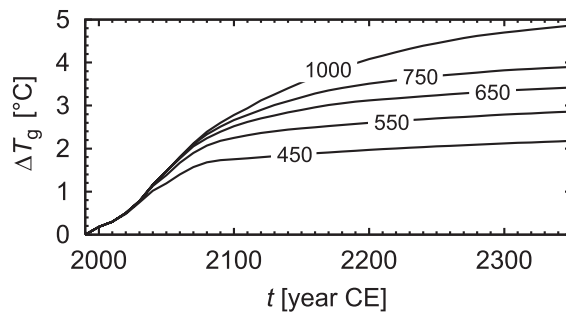
Fig. 11. Global mean temperature change \Delta T_g for the profiles WRE450, WRE550, WRE650, WRE750 and WRE1000 (stabilization scenarios for atmospheric \text{CO}_2 ), by Cubasch et al. (2001).
