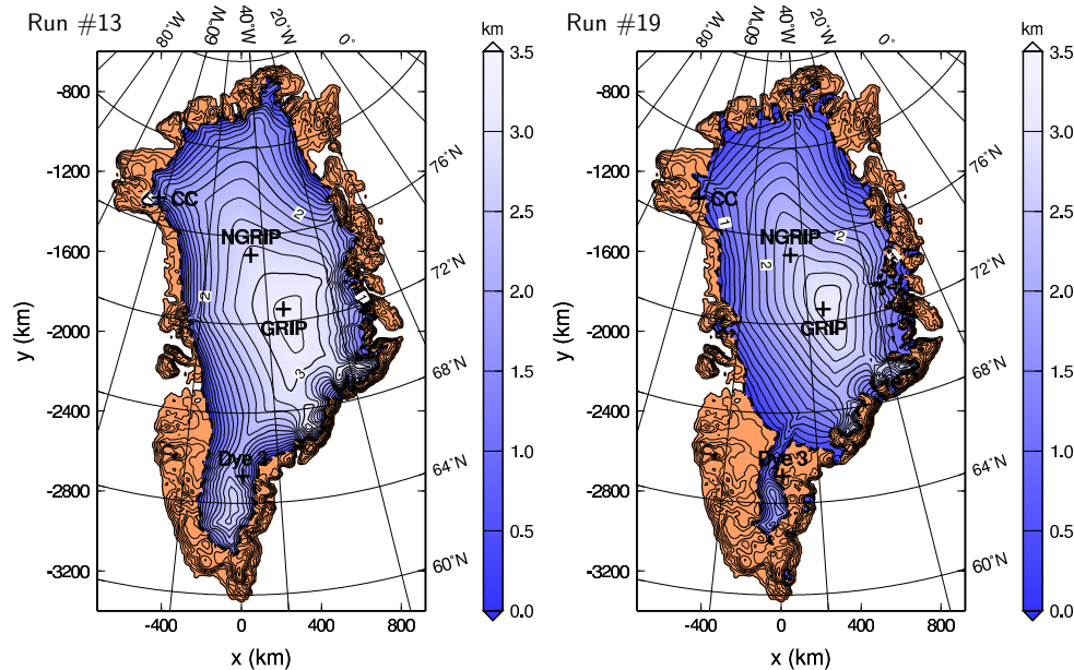
Fig. 14. Global warming runs #13 (NEGIS/ m=3 , WRE1000) and #19 (NEGIS/ m=3 , WRE1000, \gamma=5 \text{ a m}^{-1} ): Surface topography in 2350 CE. Contour spacing 200 m, labels in km a.s.l.
