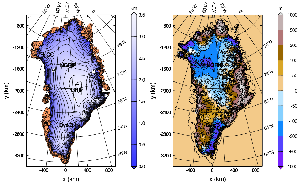
Fig. 8. Best-agreement simulation (run #3): Present-day surface topography (left panel; contour spacing 200 m, labels in km a.s.l.), and difference between simulated and observed present-day ice thickness (right panel). The heavy dashed lines indicate the simulated (left panel) and observed (right panel) ice margins.
