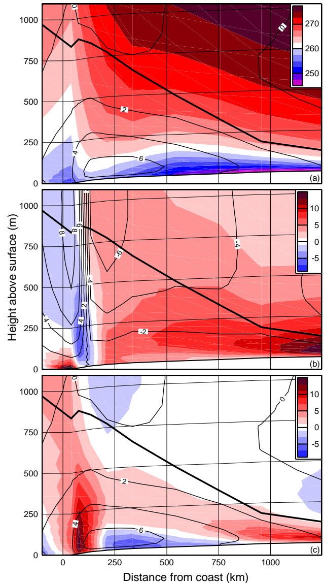
Fig. 7. Mean winter profiles for the East Antarctic sector between 30° W and 150° E. (a) potential temperature (colors in K) and along-slope wind (contours, m/s); (b) Vertical heat advection ( AdvV ) (colors, K per day) and vertical wind (contours, mm/s); (c) Horizontal (along-slope) heat advection ( AdvH ) (colors, K per day) and along-slope wind (contours, m/s). In all three figures, the surface elevation is schematically included for orientation. The thick black line represents the average ABL depth.
