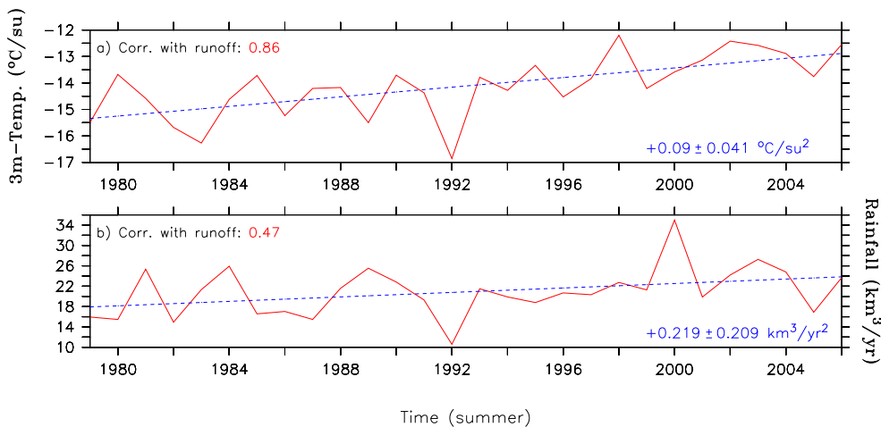
Fig. 9. Time series of the total ice sheet (a) summer (from 1 May to 30 September) temperature average (in ^\circ\text{C su}^{-1} ) and (b) yearly rainfall (in \text{km}^3 \text{ yr}^{-1} ). The correlation with the run-off (Fig. 4) is indicated as well as the trend.
