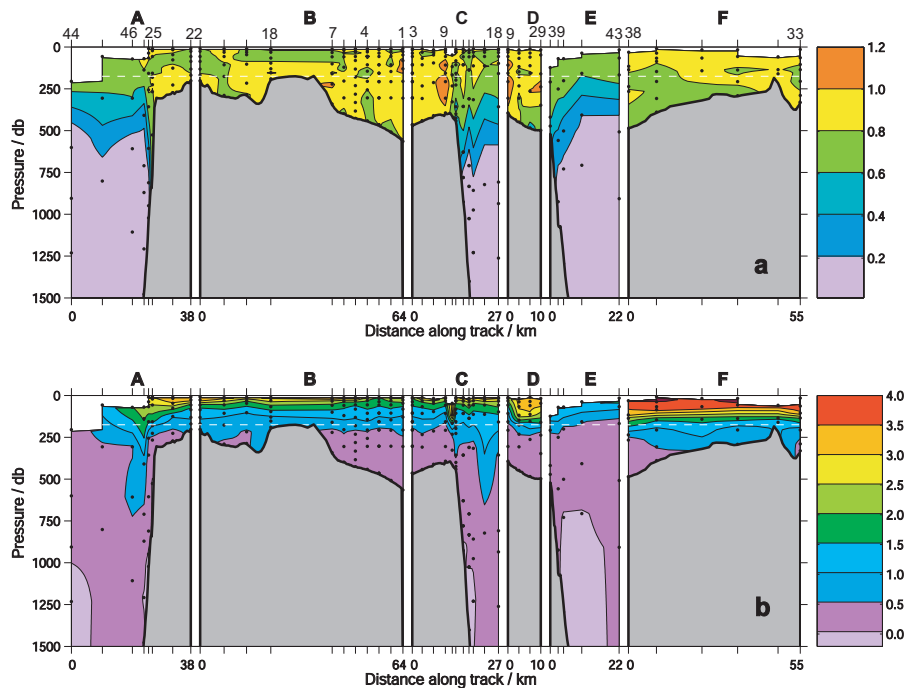
Fig. 4. (a) Meteoric water fraction (%) and (b) sea ice fraction (%) for the six hydrographic sections A to F (for locations see Fig. 1) derived from the data shown in Fig. 2. Black dots indicate bottle locations, and the depth of the base of the ice shelf is indicated by the white dashed line.
